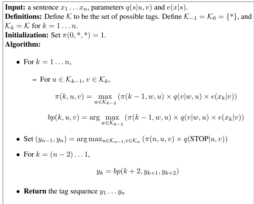
Figure 2.5: The Viterbi Algorithm with backpointers.
