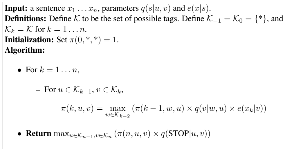
Figure 2.4: The basic Viterbi Algorithm.
